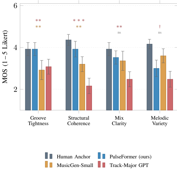
Fig. 4. MOS results ( N = 25 , 95% CI; Wilcoxon vs. PulseFormer). Stars above bars: sig. vs. MGen / TM-GPT : *** p < 0.001 ; ** p < 0.01 ; ^\dagger p < 0.10 ; ns. PF \approx Human Anchor (GT, p = 0.93 ); dominates SC ( p < 0.001 , d > 1.9 ).
