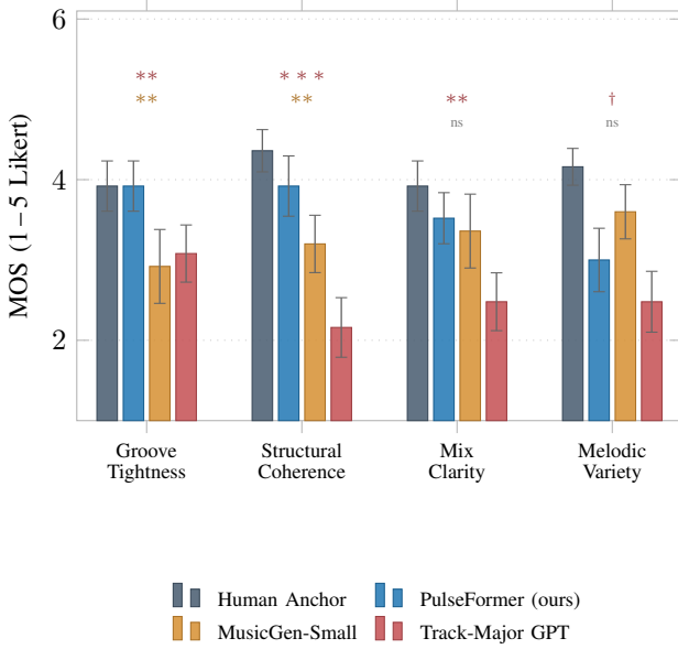
Fig. 4. MOS results ( N = 25 , 95 % CI; Wilcoxon vs. PulseFormer). Stars above bars: sig. vs. MG / TM-GPT : *** p < 0.001 ; ** p < 0.01 ; † p < 0.10 ; ns. PF \approx Human Anchor (GT, p = 0.93 ); dominates SC ( p < 0.001 , d > 1.9 ).
