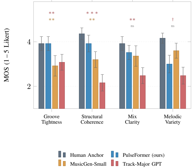
Fig. 4. MOS results ( N = 25 , 95% CI; Wilcoxon vs. PulseFormer). Stars above bars: sig. vs. MG en / TM -GPT: *** p < 0.001 ; ** p < 0.01 ; ^\dagger p < 0.10 ; ns. PF \approx Human Anchor (GT, p = 0.93 ); dominates SC ( p < 0.001 , d > 1.9 ).
