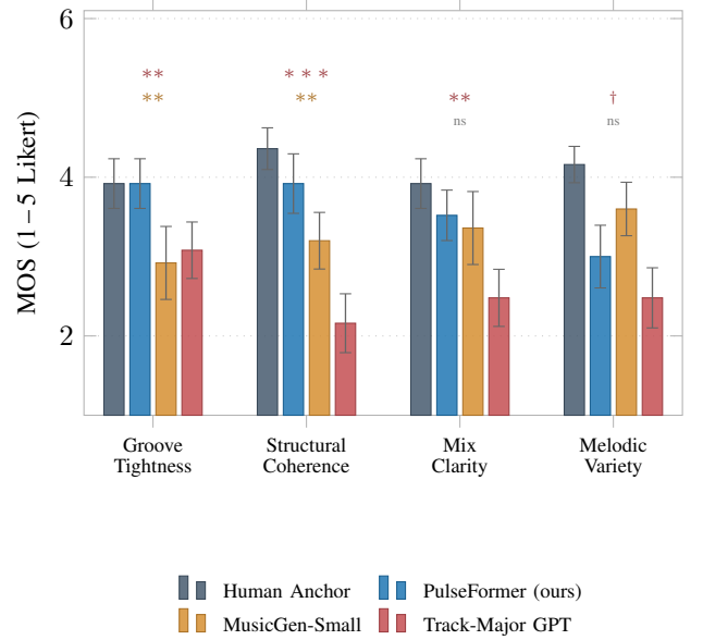
Fig. 4. MOS results ( N = 25 , 95% CI; Wilcoxon vs. PulseFormer). Stars above bars: sig. vs. MGen / TM-GPT : *** p < 0.001 ; ** p < 0.01 ; ^\dagger p < 0.10 ; ns. PF \approx Human Anchor (GT, p = 0.93 ); dominates SC ( p < 0.001 , d > 1.9 ).
