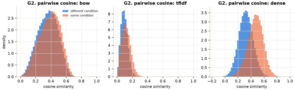
Figure 7: Pairwise cosine similarity for same-condition vs different-condition pairs: only the dense model separates the two distributions.
