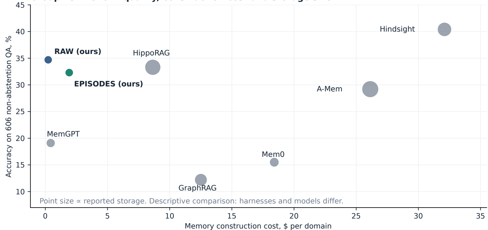
GroupMemBench · quality, construction cost and storage size
