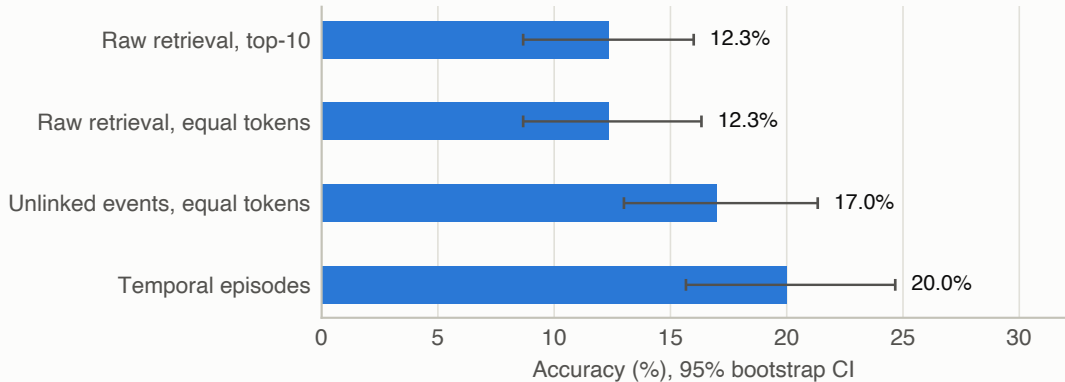
EverMemBench Temporal Duration questions (n = 300)
