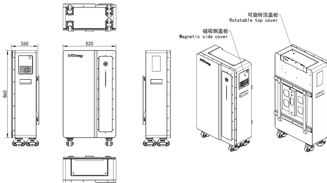
图 2 电池包尺寸图 Figure 2 The dimensions of battery pack
