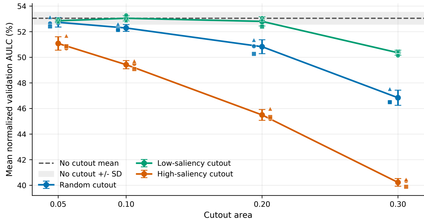
CIFAR-100, M4: Normalized validation AULC versus cutout area
