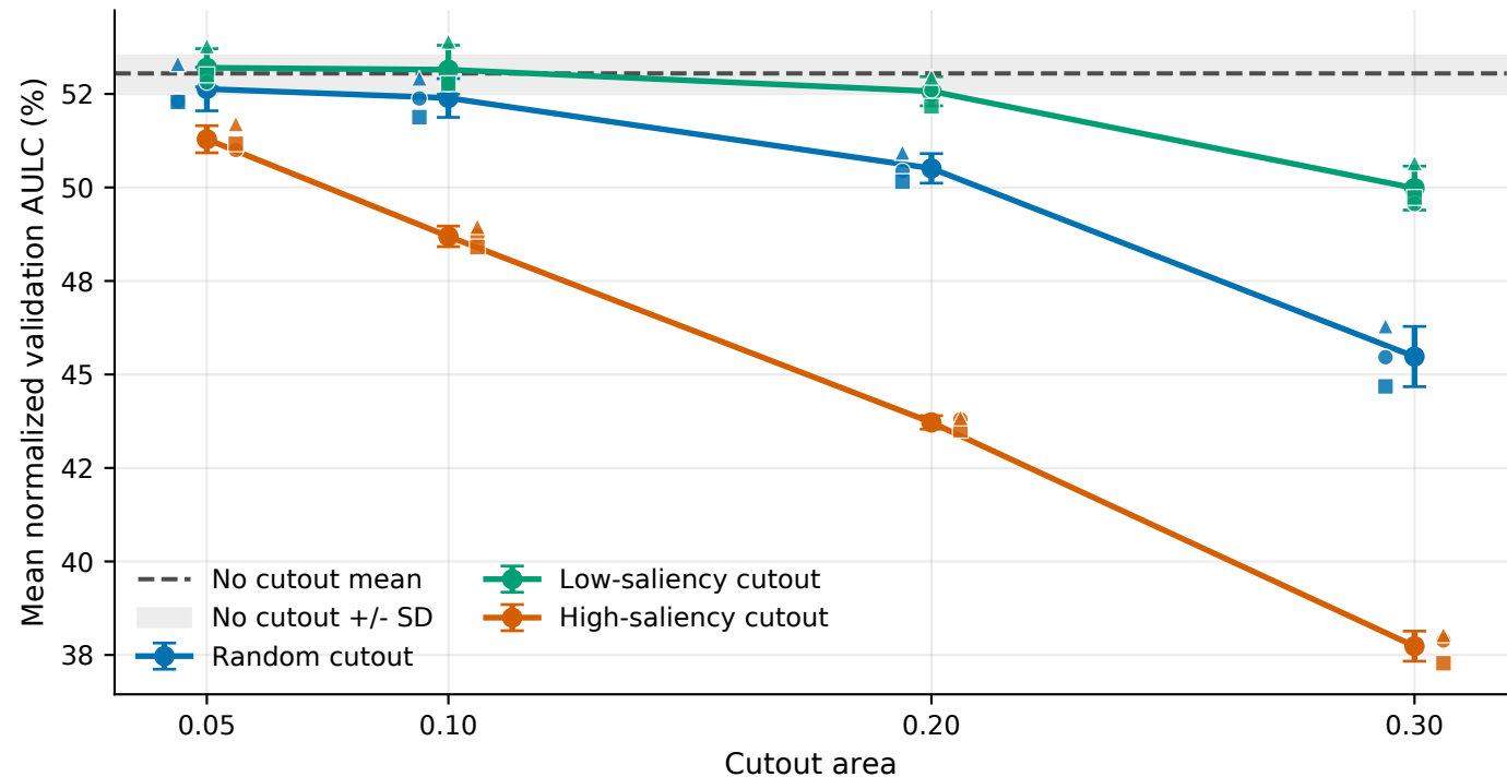
CIFAR-100, M8: Normalized validation AULC versus cutout area
