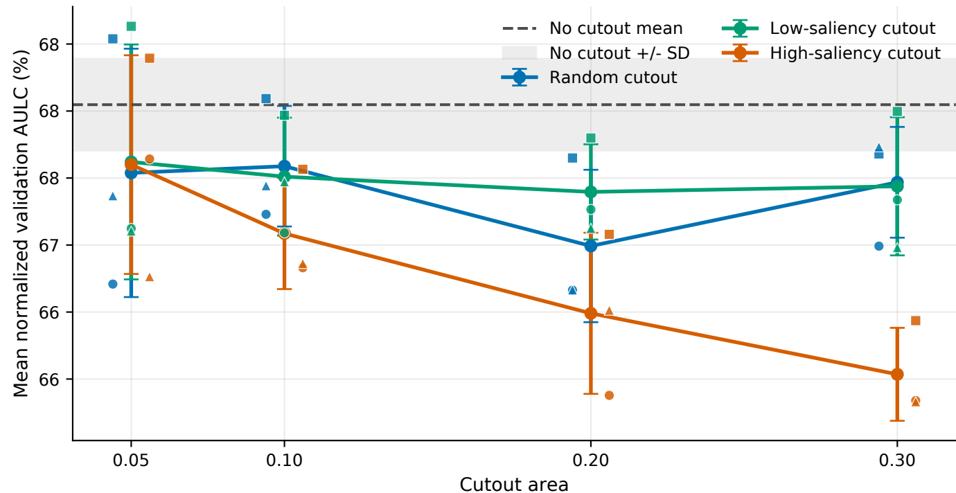
RawMal-TF, M4: Normalized validation AULC versus cutout area
