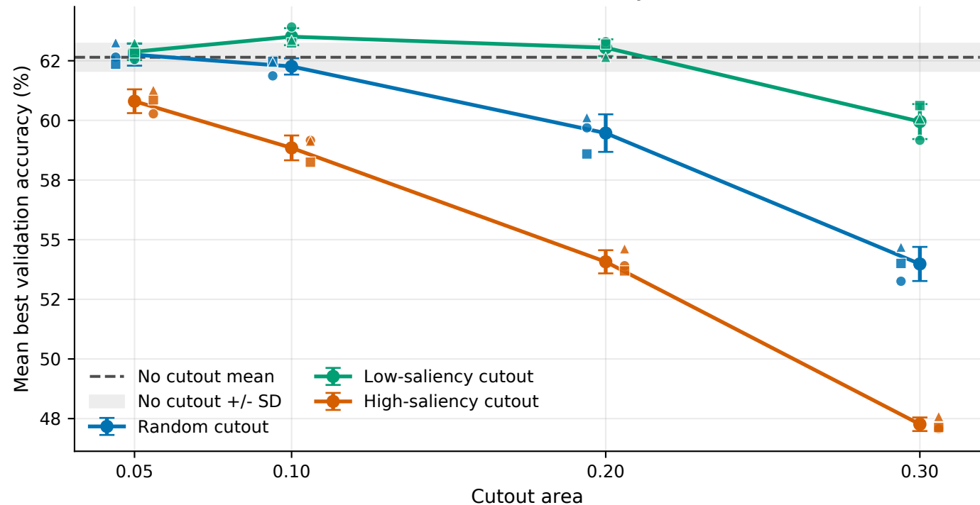
CIFAR-100, M4: Best validation accuracy versus cutout area
