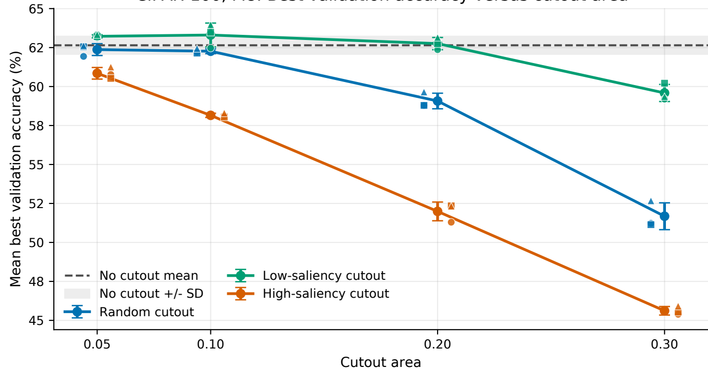
CIFAR-100, M8: Best validation accuracy versus cutout area
