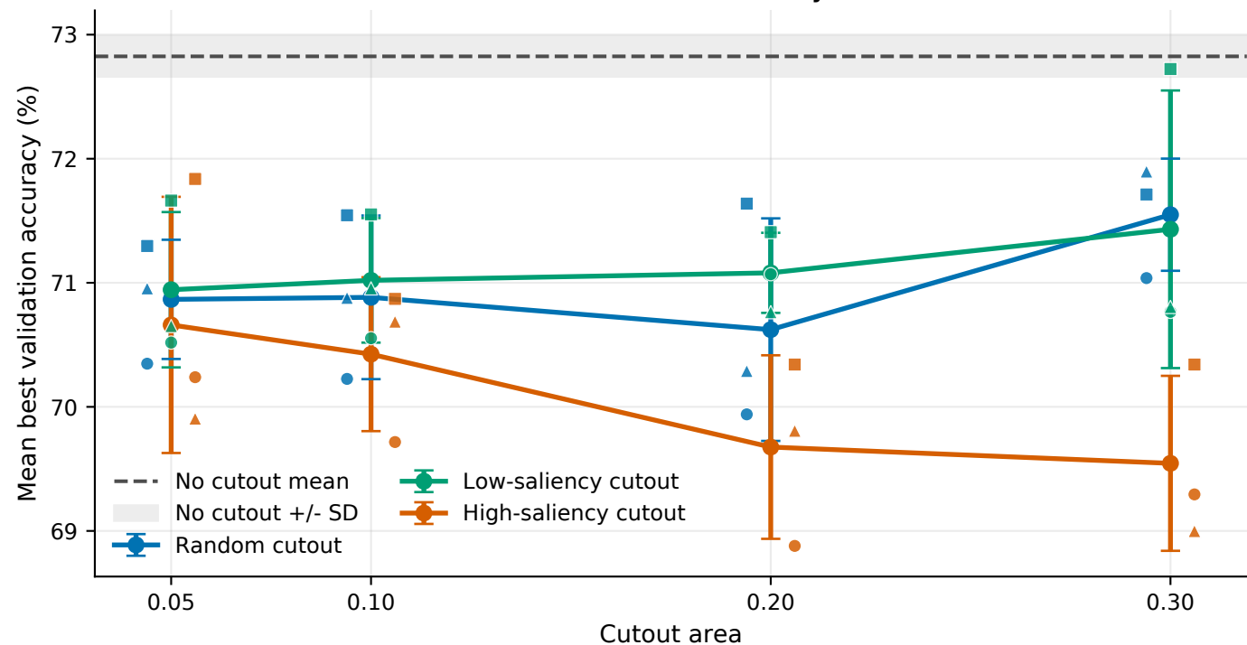
RawMal-TF, M4: Best validation accuracy versus cutout area
