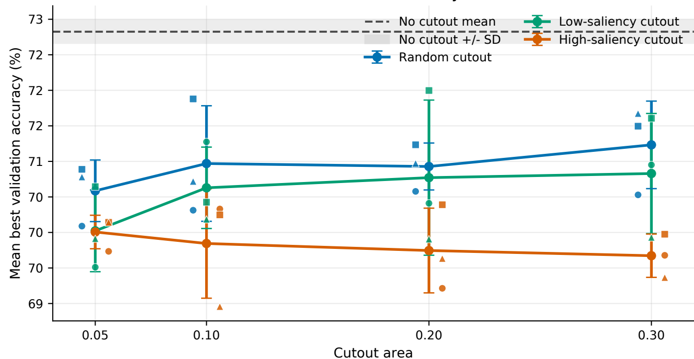
RawMal-TF, M8: Best validation accuracy versus cutout area
