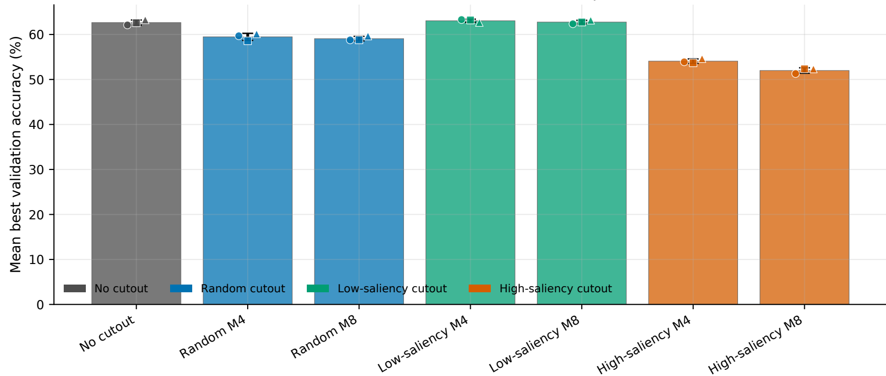
CIFAR-100, area 0.20: condition comparison
