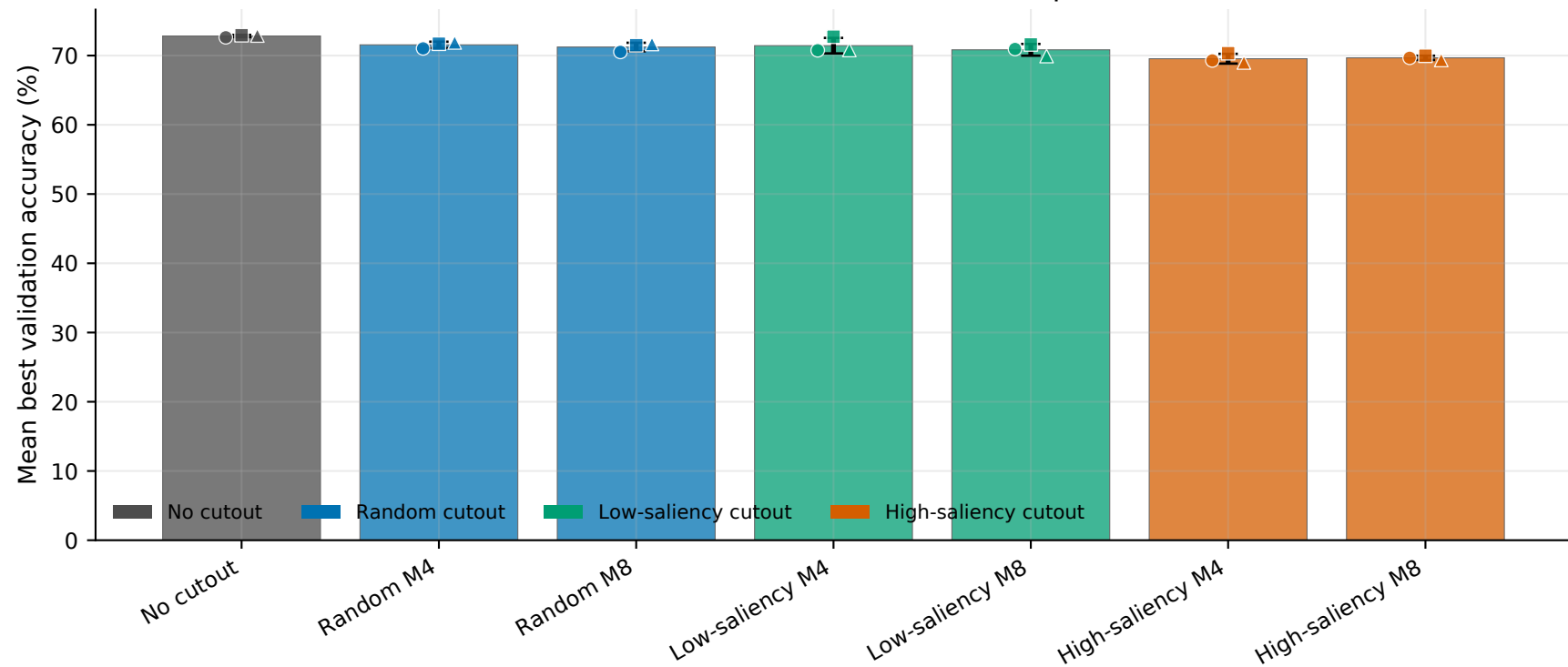
RawMal-TF, area 0.30: condition comparison
