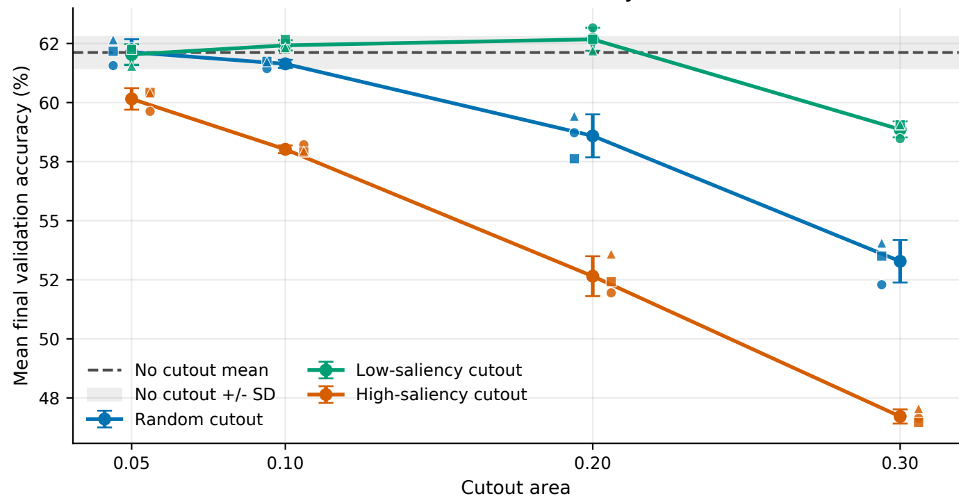
CIFAR-100, M4: Final validation accuracy versus cutout area
