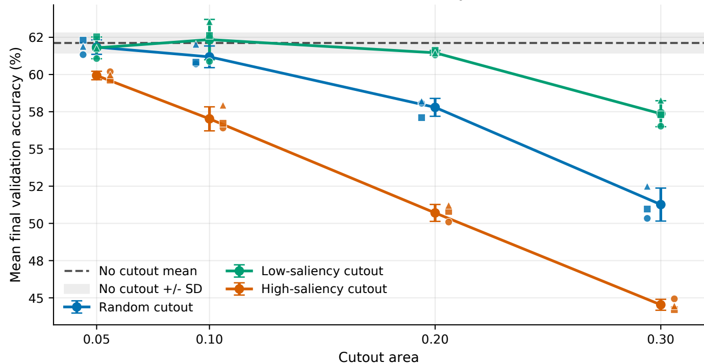
CIFAR-100, M8: Final validation accuracy versus cutout area
