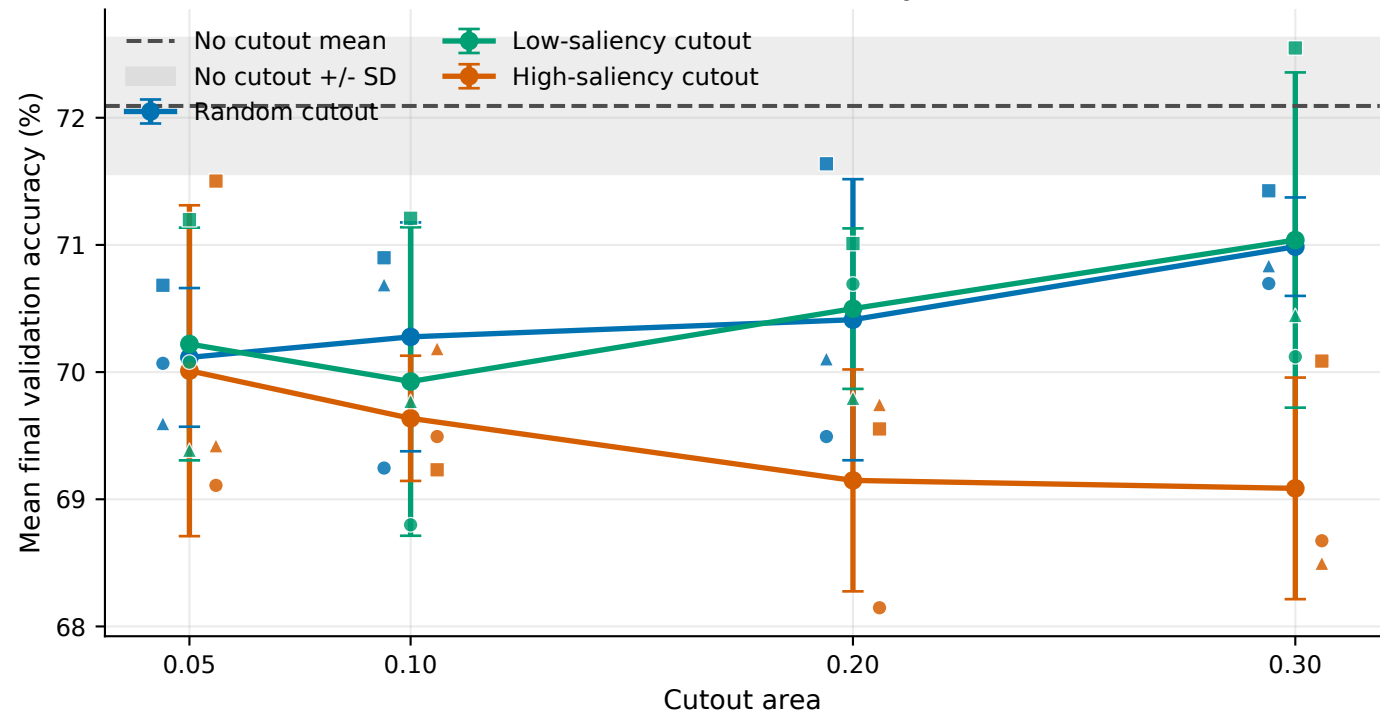
RawMal-TF, M4: Final validation accuracy versus cutout area
