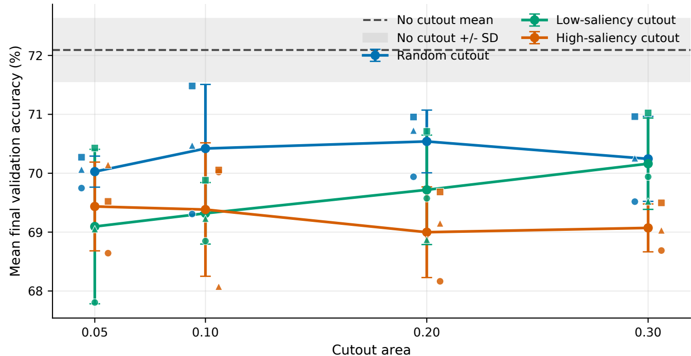
RawMal-TF, M8: Final validation accuracy versus cutout area
