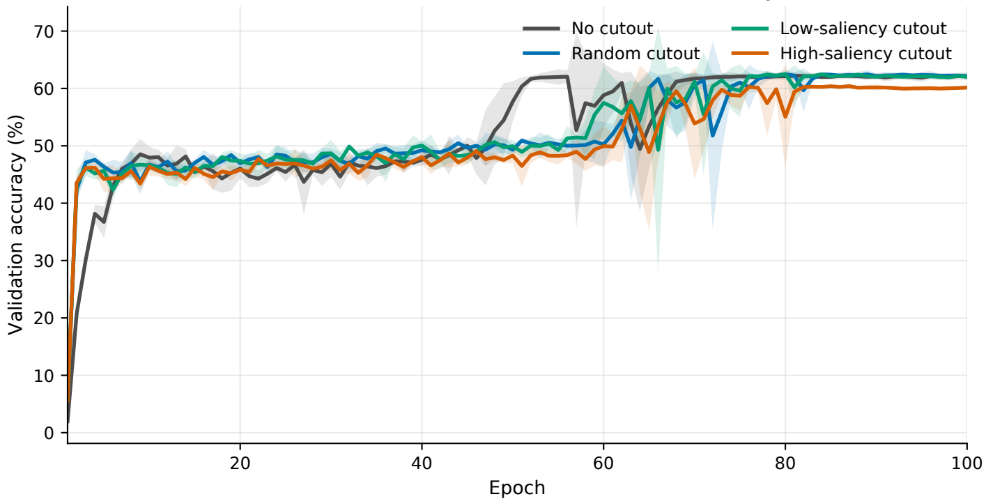
CIFAR-100, M4, area 0.05: mean validation accuracy curve
