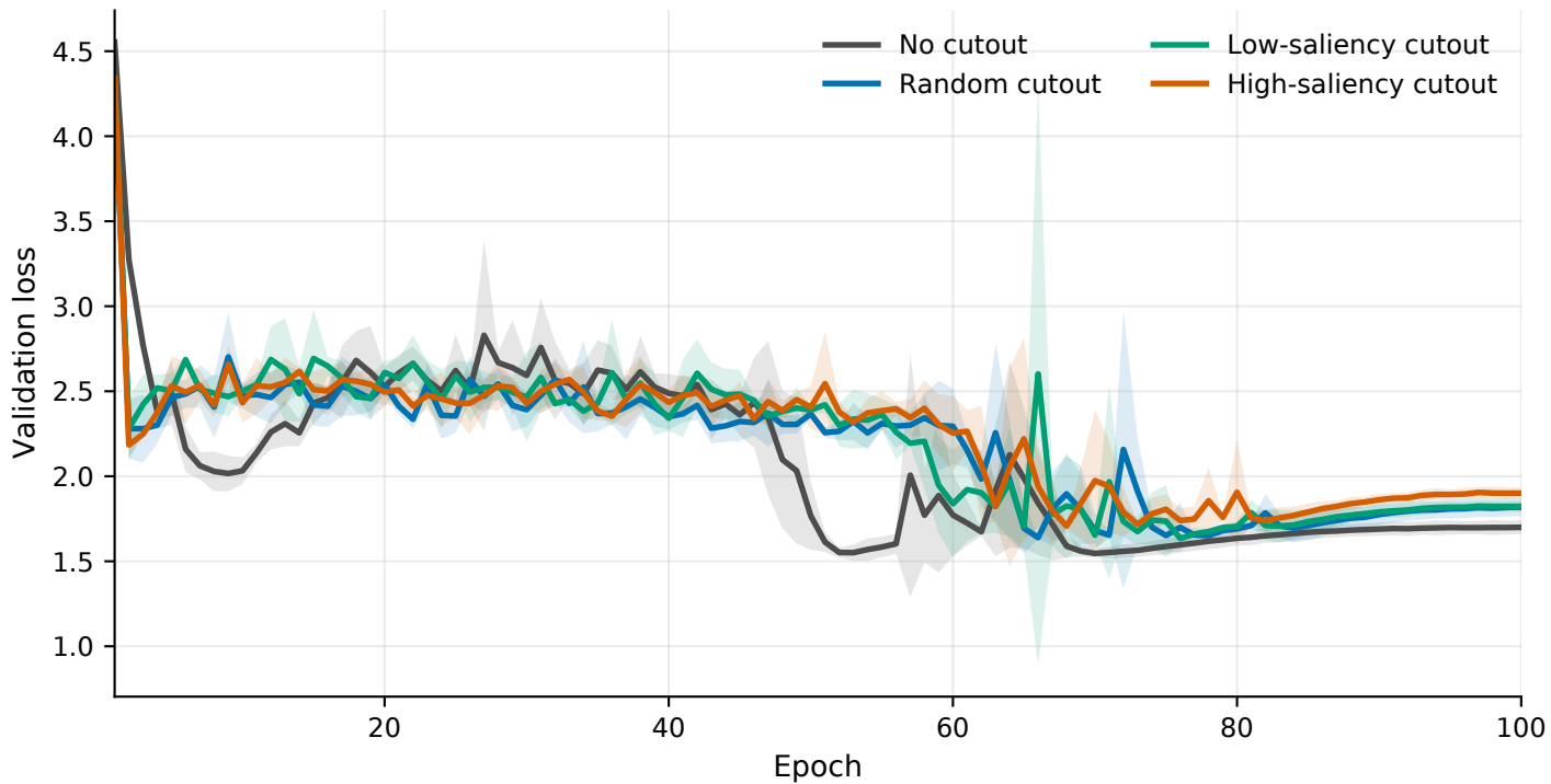
CIFAR-100, M4, area 0.05: mean validation loss curve
