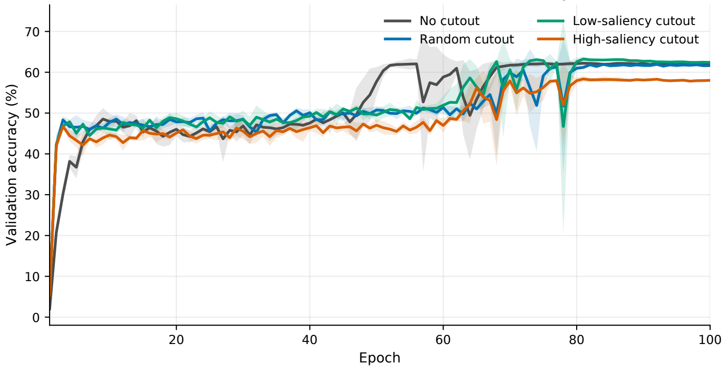
CIFAR-100, M4, area 0.10: mean validation accuracy curve
