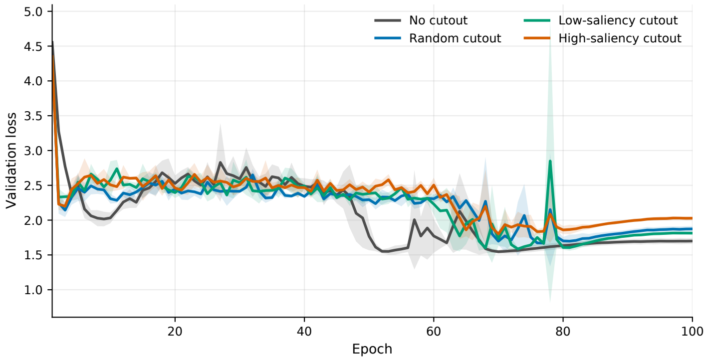
CIFAR-100, M4, area 0.10: mean validation loss curve
