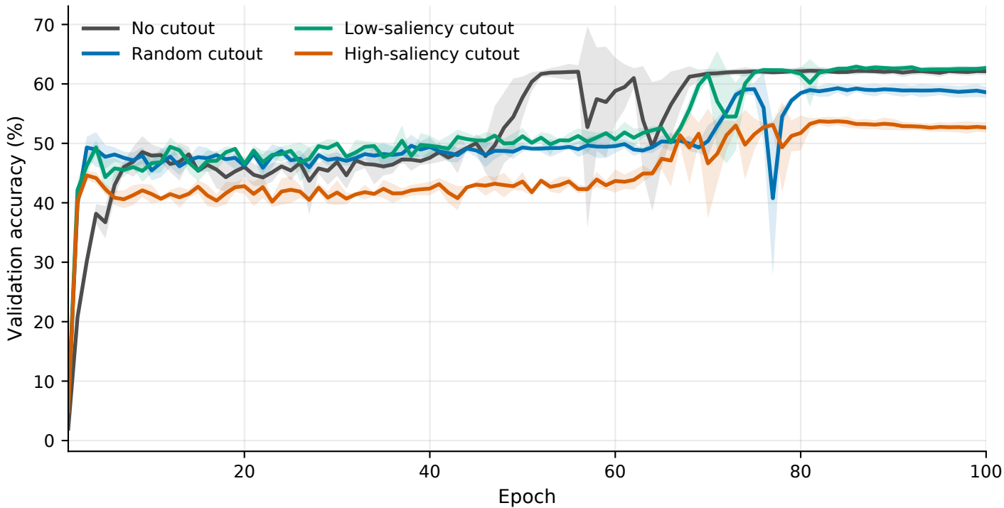
CIFAR-100, M4, area 0.20: mean validation accuracy curve
