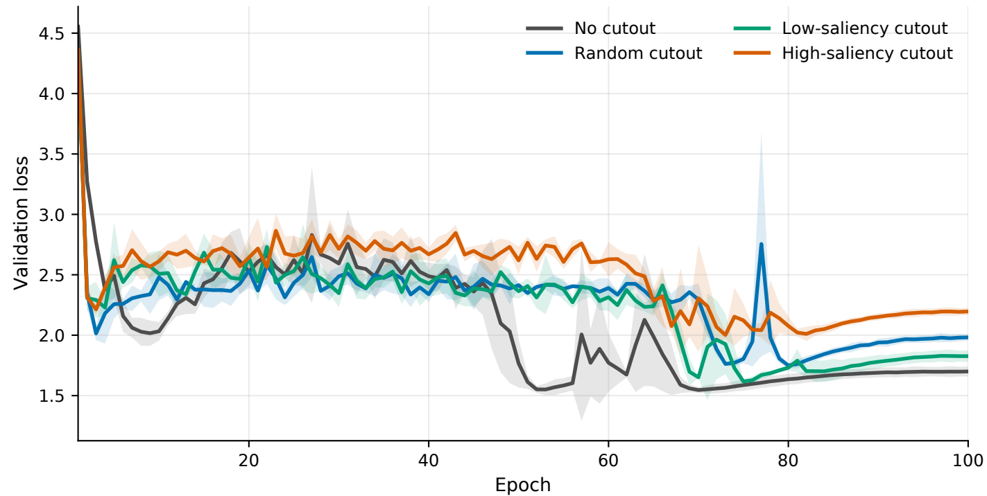
CIFAR-100, M4, area 0.20: mean validation loss curve
