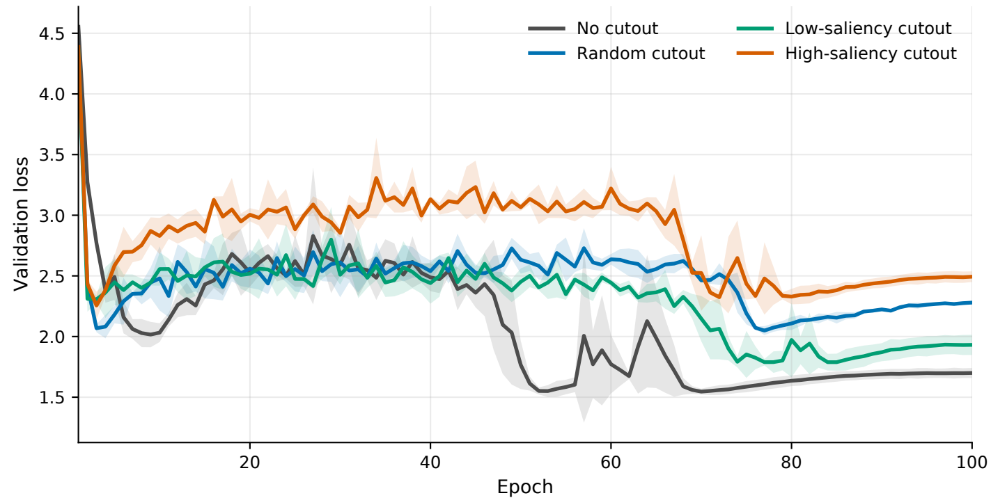
CIFAR-100, M4, area 0.30: mean validation loss curve
