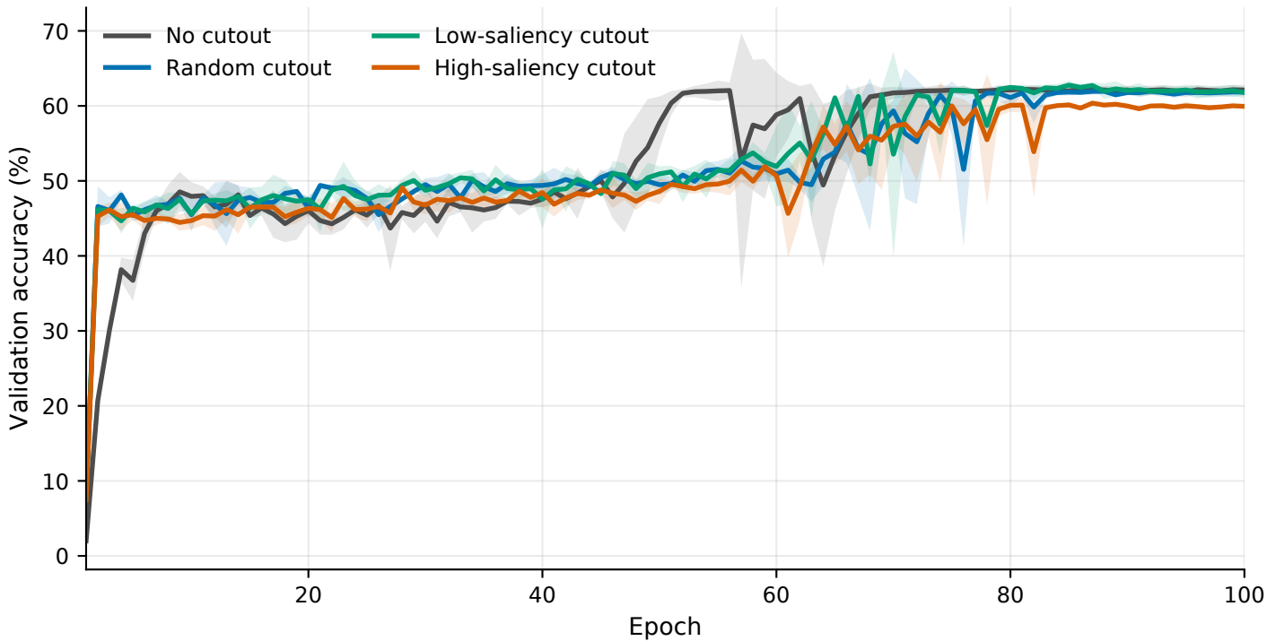
CIFAR-100, M8, area 0.05: mean validation accuracy curve
