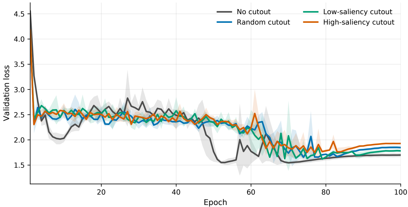
CIFAR-100, M8, area 0.05: mean validation loss curve
