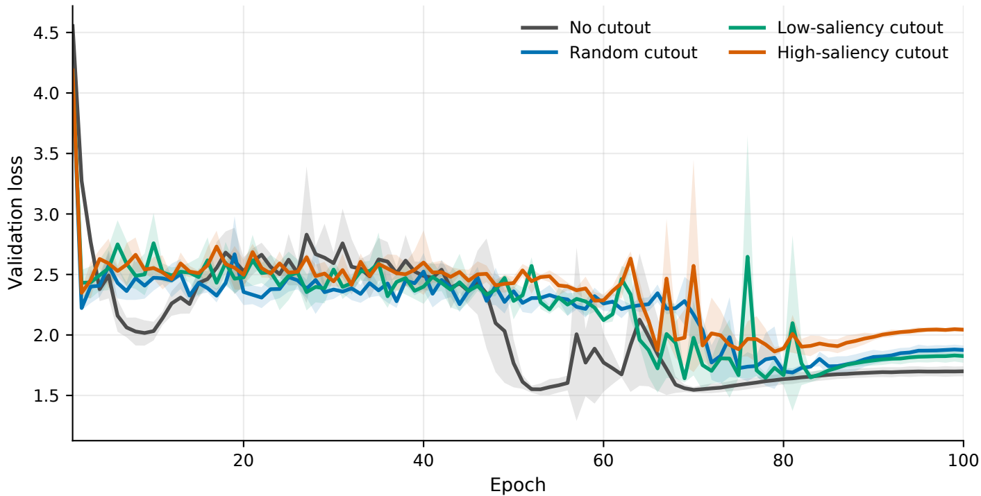
CIFAR-100, M8, area 0.10: mean validation loss curve
