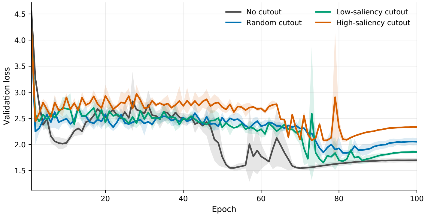
CIFAR-100, M8, area 0.20: mean validation loss curve
