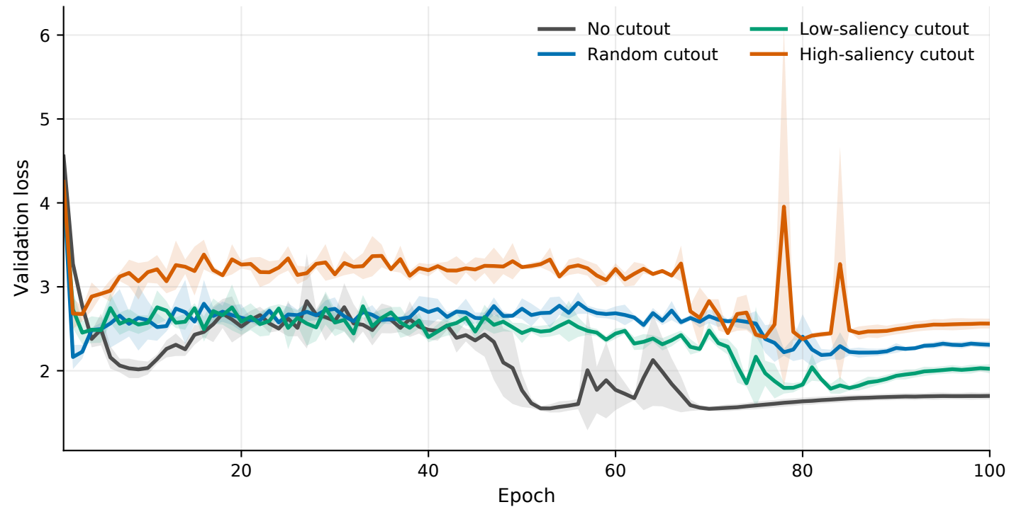
CIFAR-100, M8, area 0.30: mean validation loss curve
