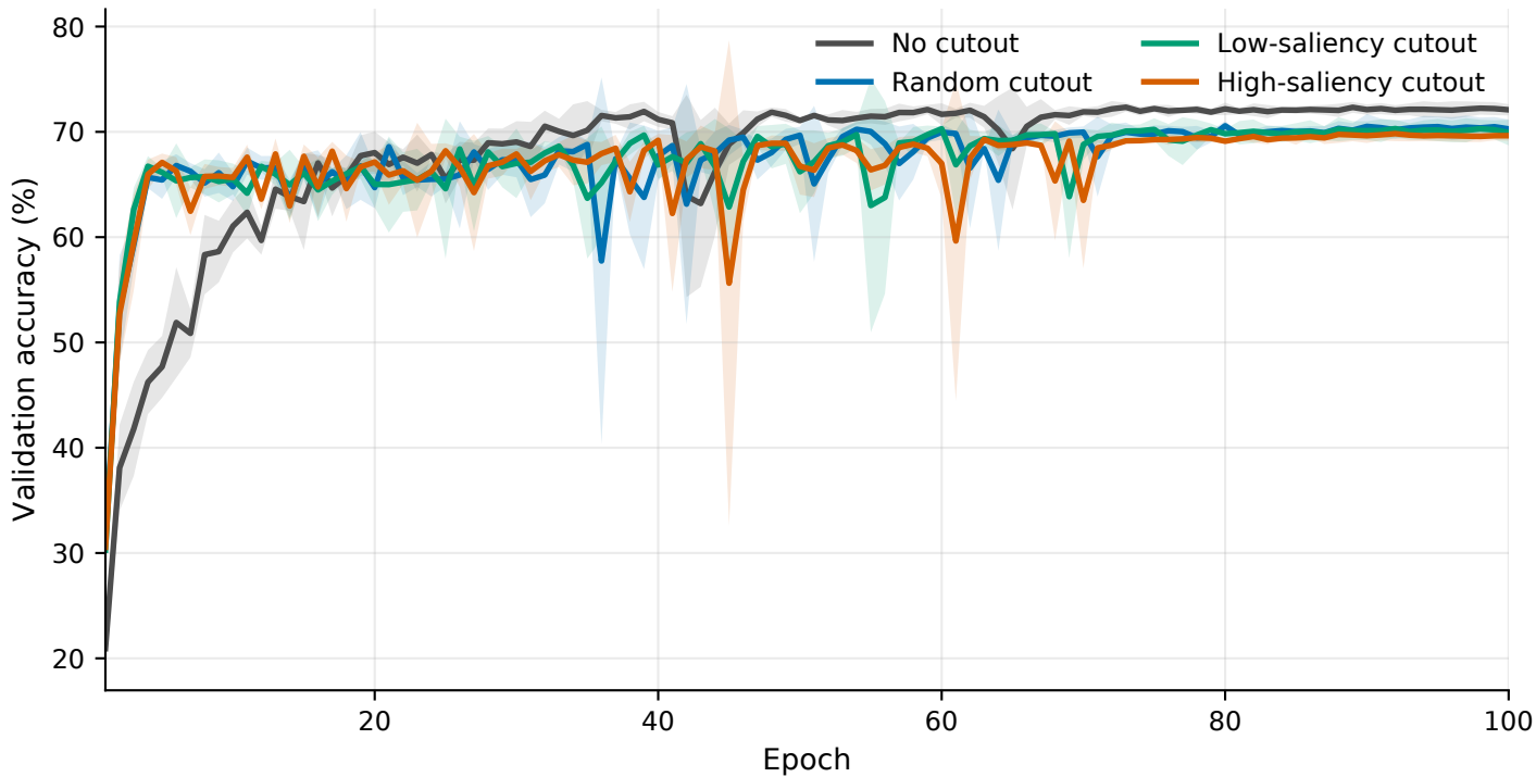
RawMal-TF, M4, area 0.10: mean validation accuracy curve
