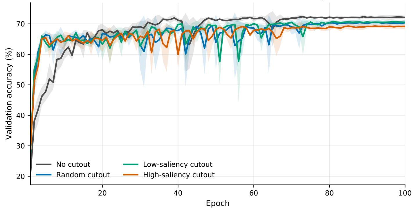
RawMal-TF, M4, area 0.20: mean validation accuracy curve
