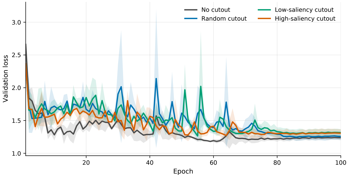
RawMal-TF, M4, area 0.20: mean validation loss curve
