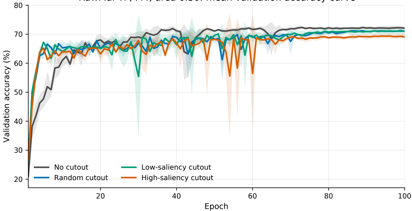
RawMal-TF, M4, area 0.30: mean validation accuracy curve
