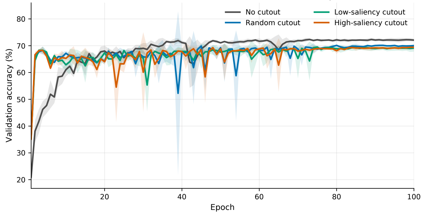
RawMal-TF, M8, area 0.05: mean validation accuracy curve
