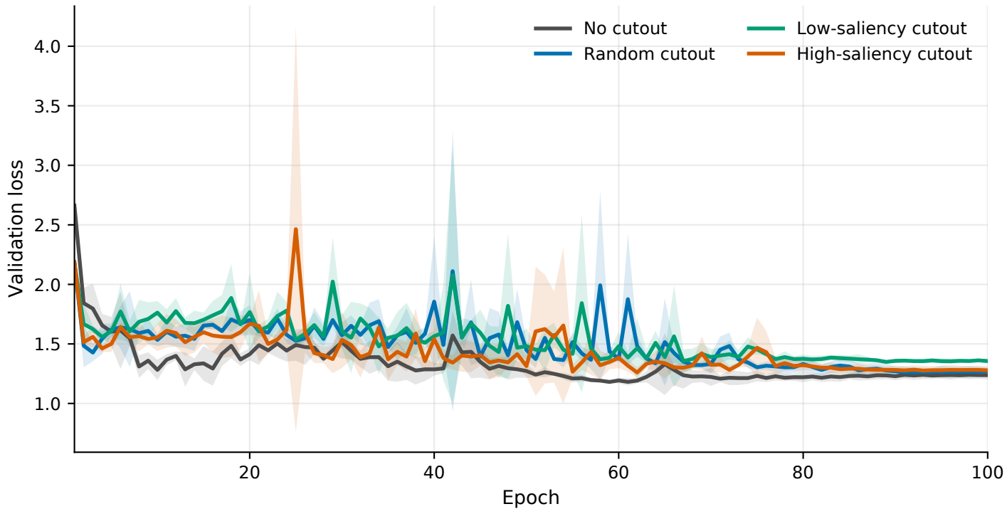
RawMal-TF, M8, area 0.10: mean validation loss curve
