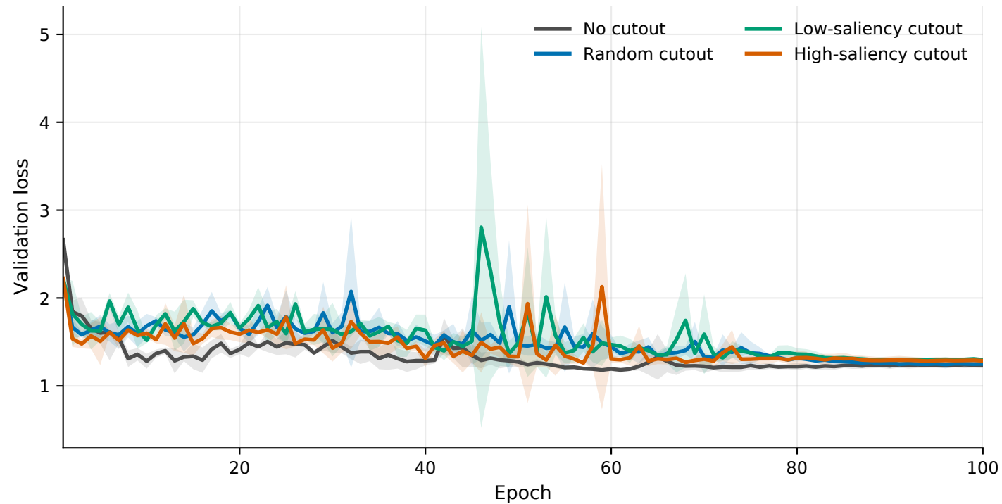
RawMal-TF, M8, area 0.20: mean validation loss curve
