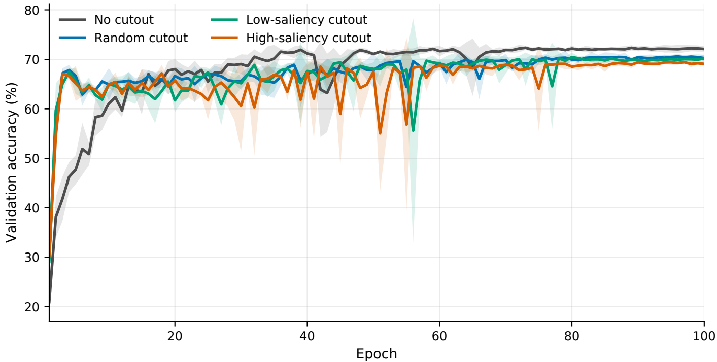
RawMal-TF, M8, area 0.30: mean validation accuracy curve
