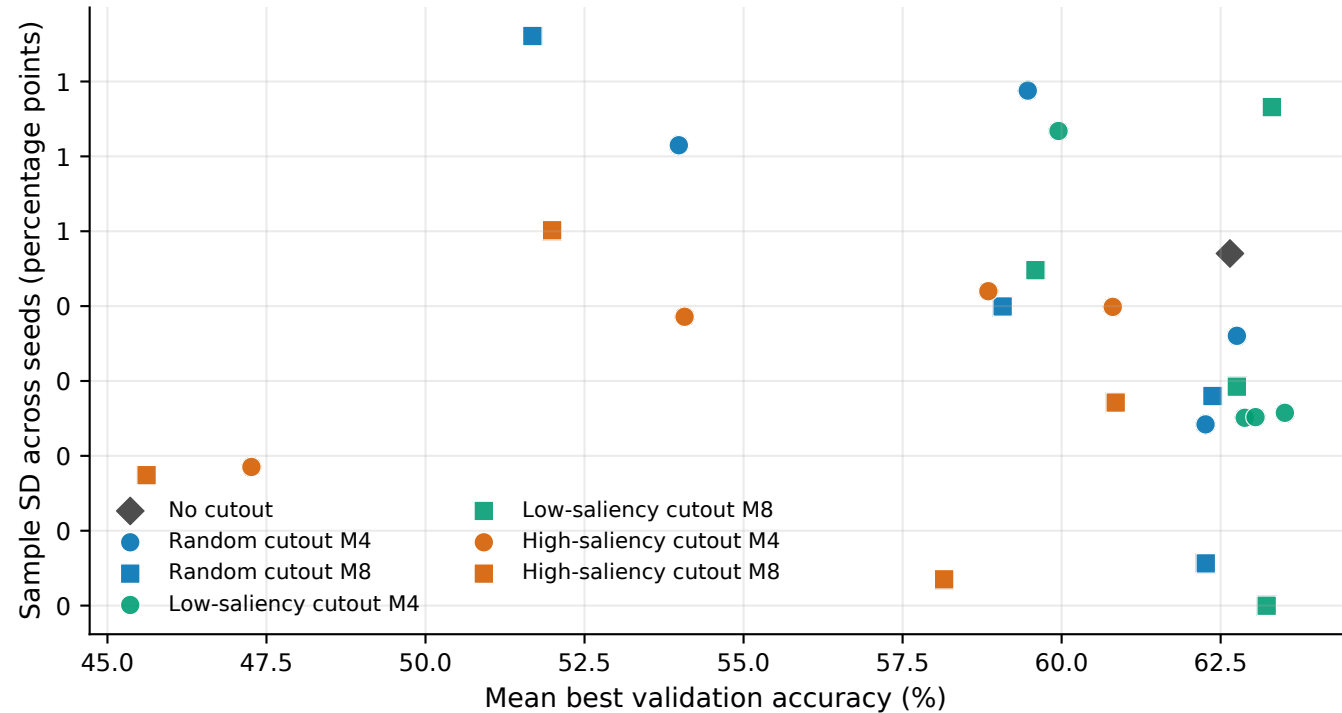
CIFAR-100: mean performance versus across-seed variability
