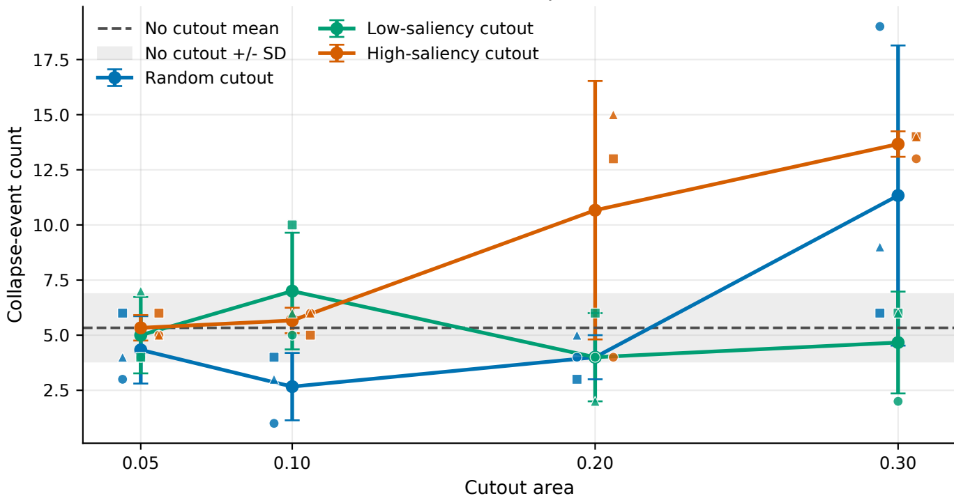
CIFAR-100, M8: Collapse-event count
