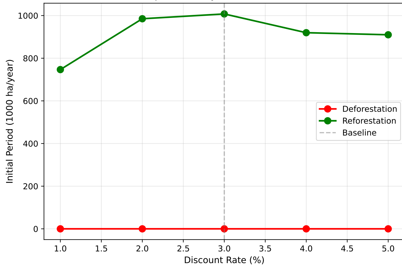
Optimal Policy vs Discount Rate
