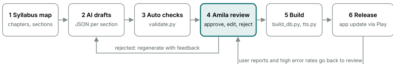
Figure 2 – Content pipeline
