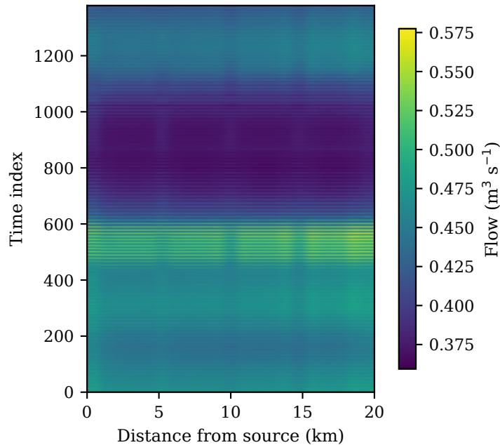
Reconstructed field
