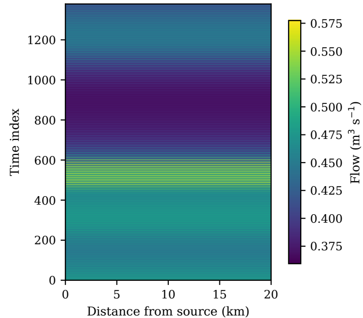
Reference field
