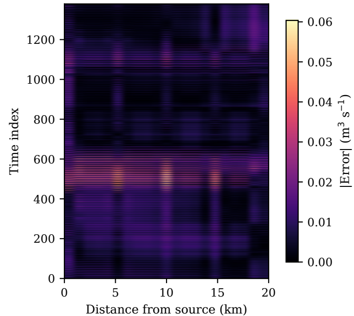
Absolute-error field
