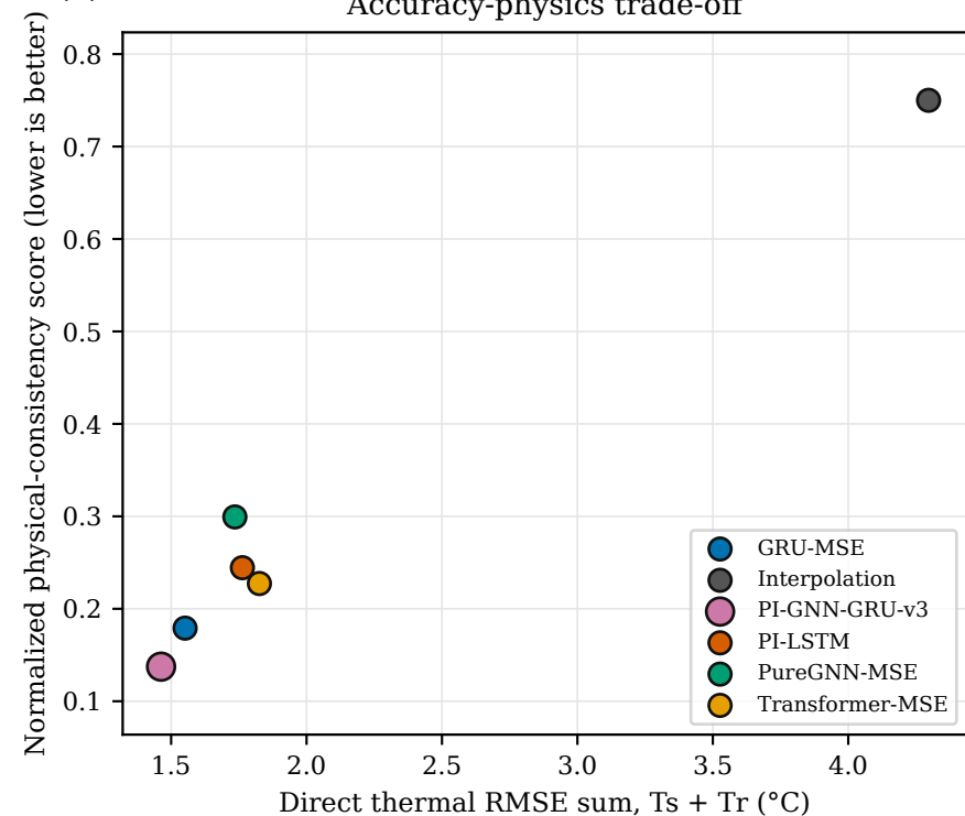
Accuracy-physics trade-off
