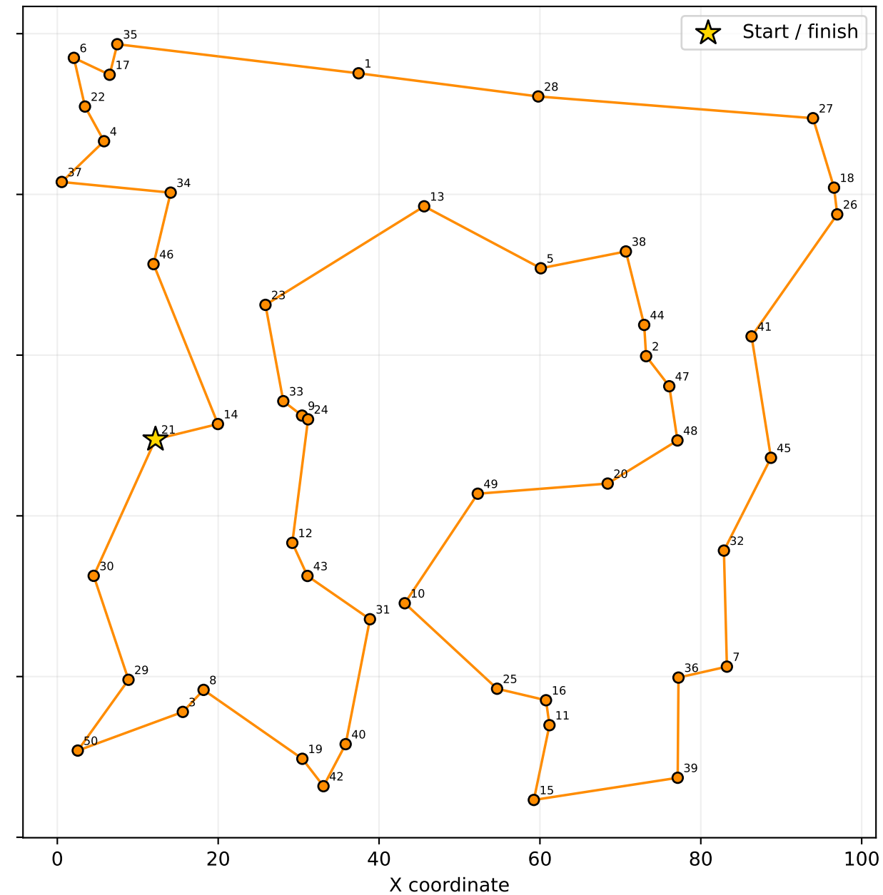
GA — Best Observed 50-City Route Seed 47, distance 576.75
