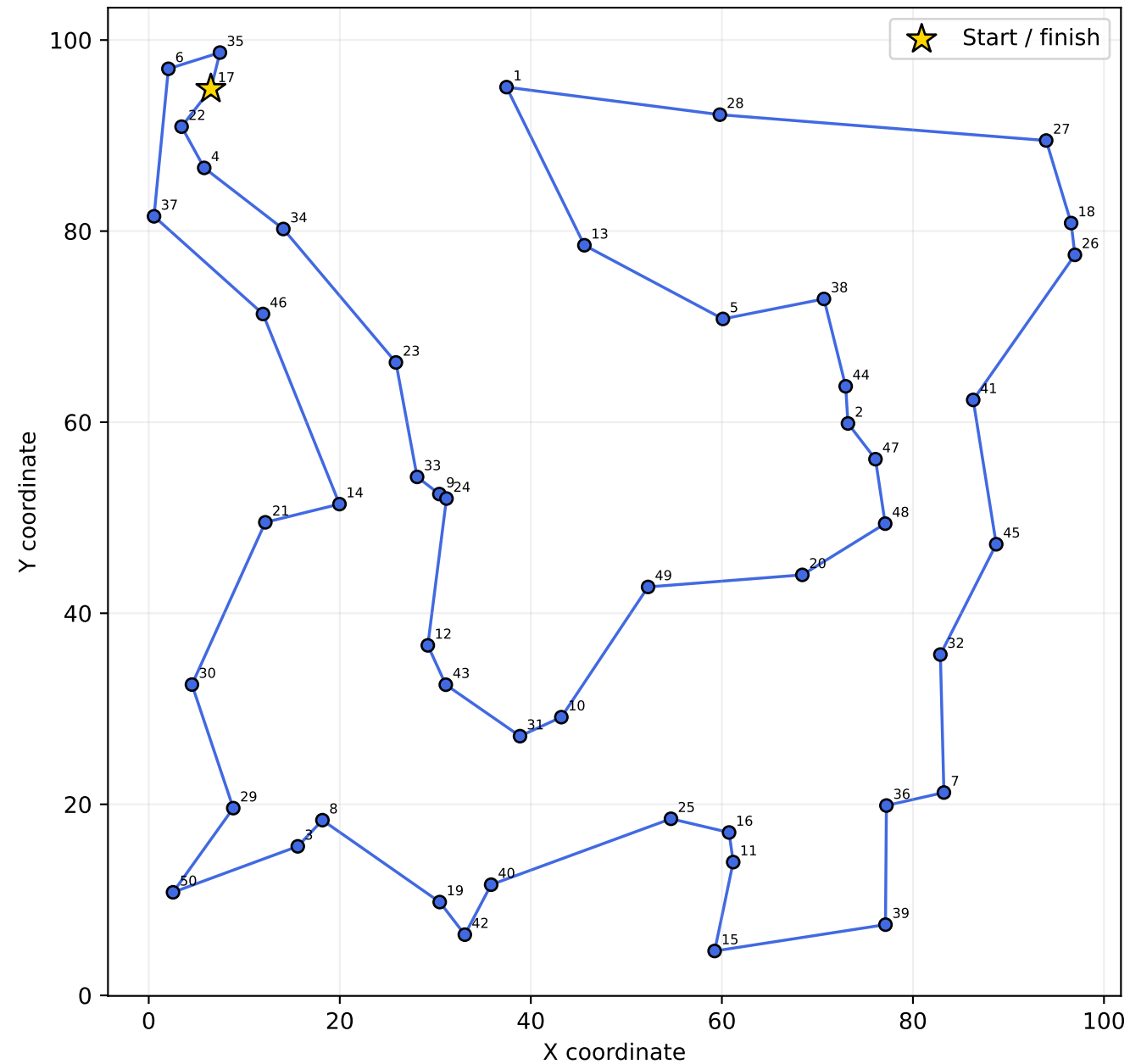
ILS — Best Observed 50-City Route Seed 50, distance 564.13
