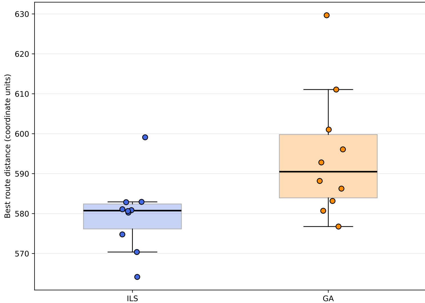
50-City Results — All 10 Runs per Algorithm
