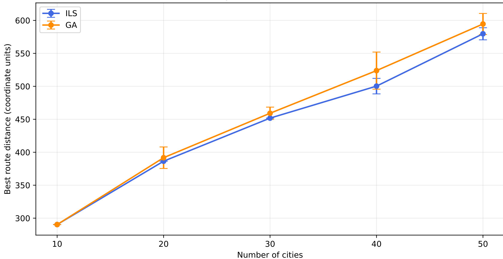
Solution Quality — Mean \pm 1 SD Across 10 Runs
